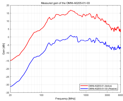
Figure 1: Measured gain (OMNI-A0205-01/-03 (Passive))
