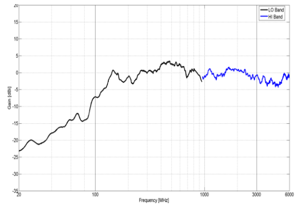
Figure 2: Measured gain (OMNI-A0205-02)
